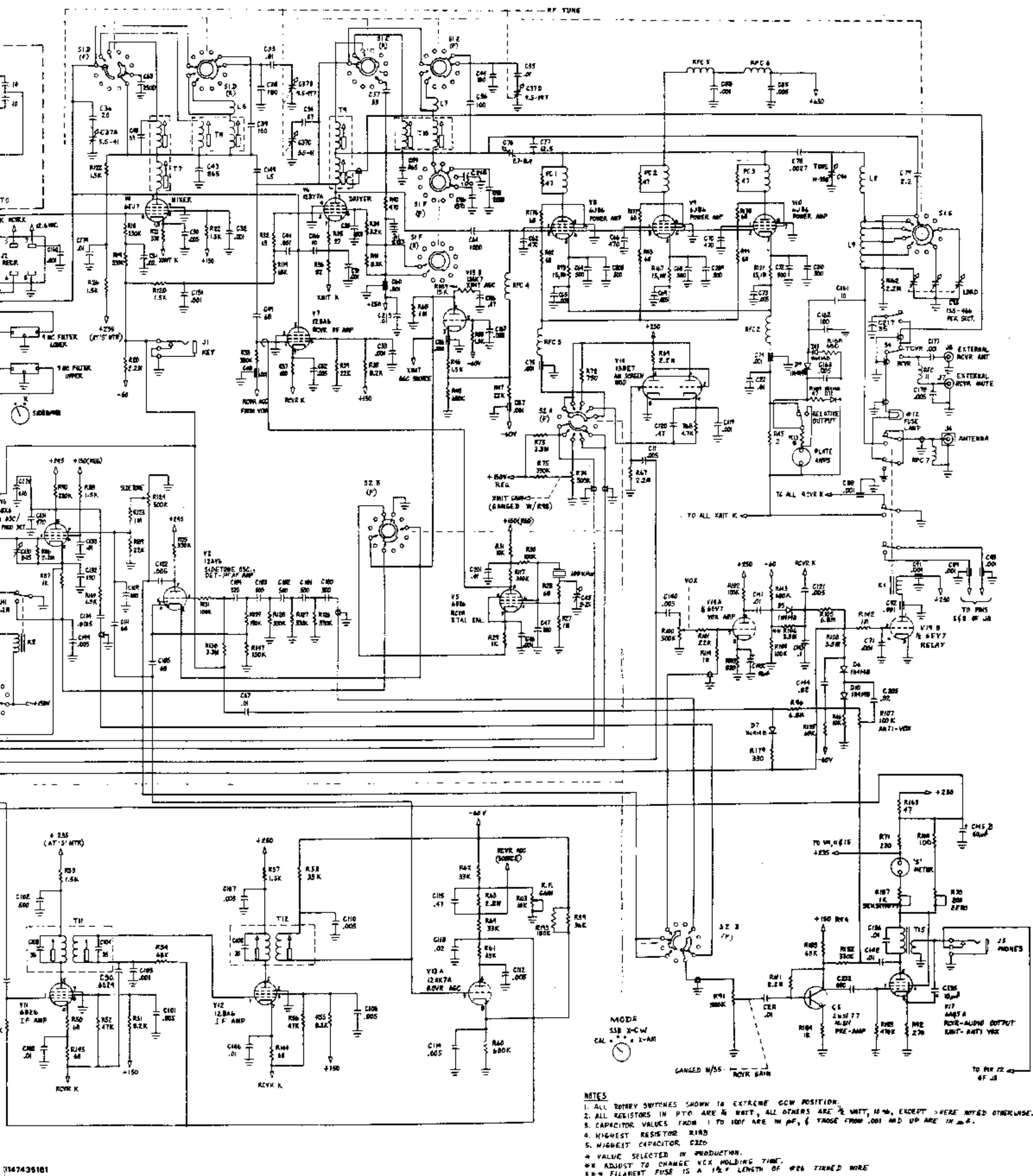
Figure 5-5. TR-4C Schematic
